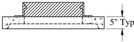
Optional 24" Cast Iron Frame & Cover
